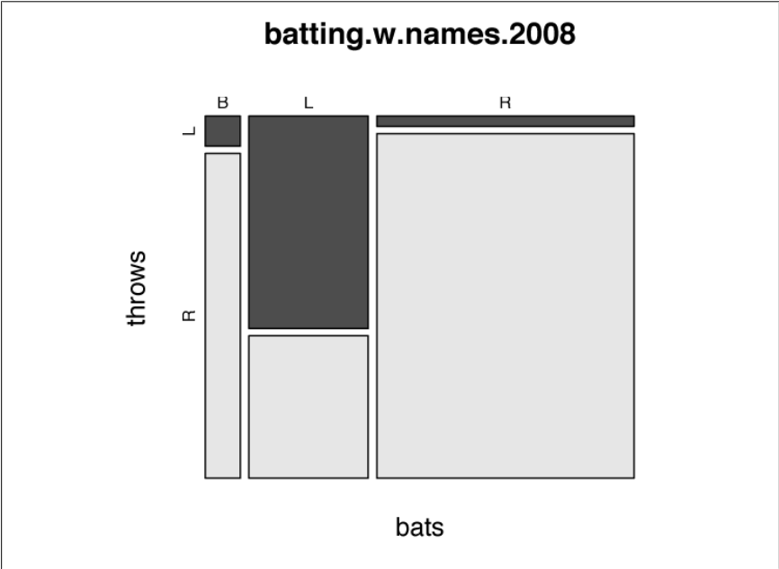
Figure 14-12. Mosaic plot
