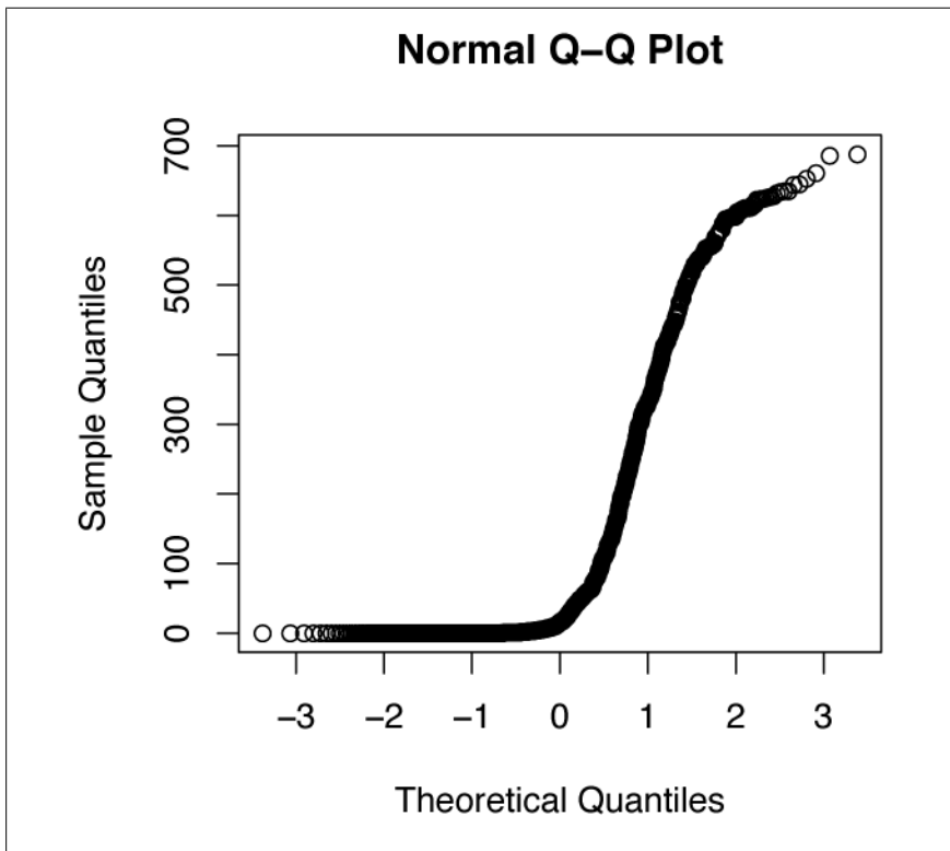
Figure 14-21. Quantile-quantile plot
